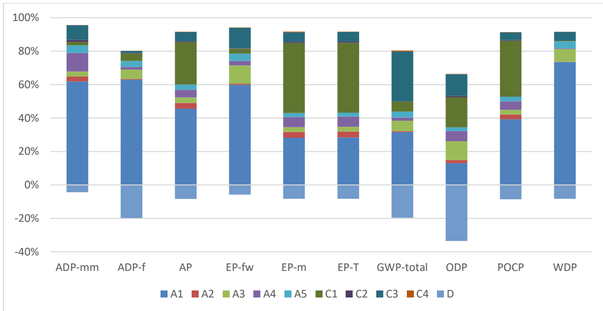
Figure 2: Tensor® TriAx® TXR - Impact of the individual modules on the environmental core indicators
