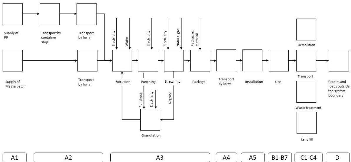
Figure 1: Process flow chart of the production of Tensor® TriAx®
